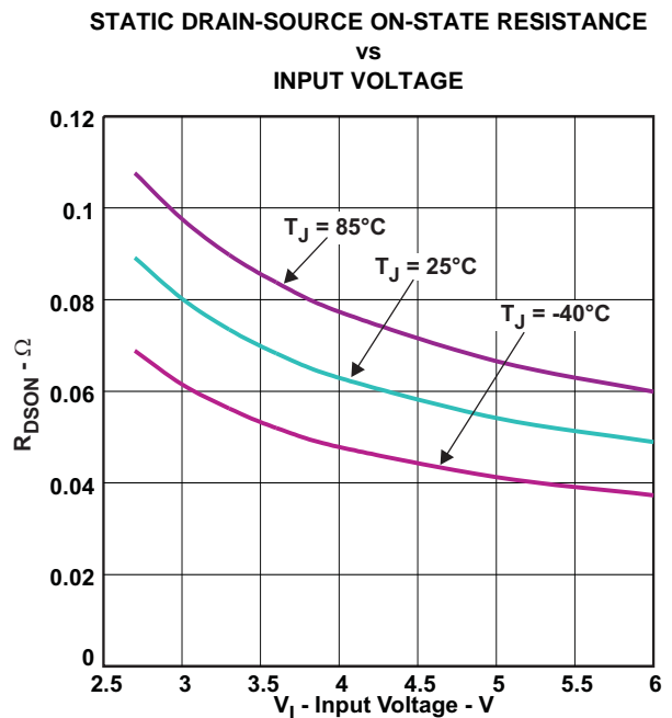
Figure 10. Low-Side Switch
